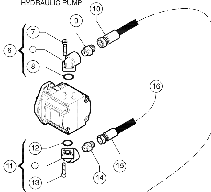
HYDRAULIC PUMP
